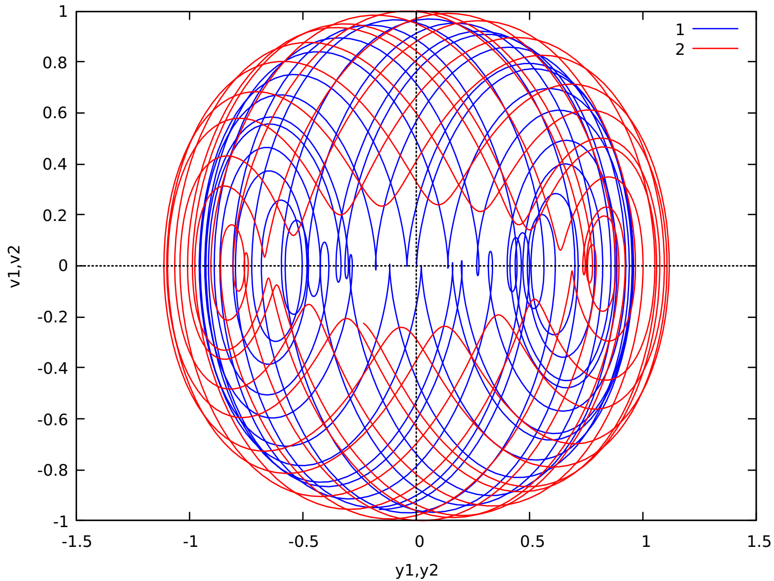
Coupled oscillators
