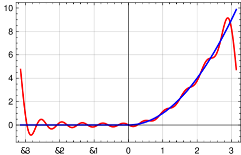
Convergence of Fourier Series
