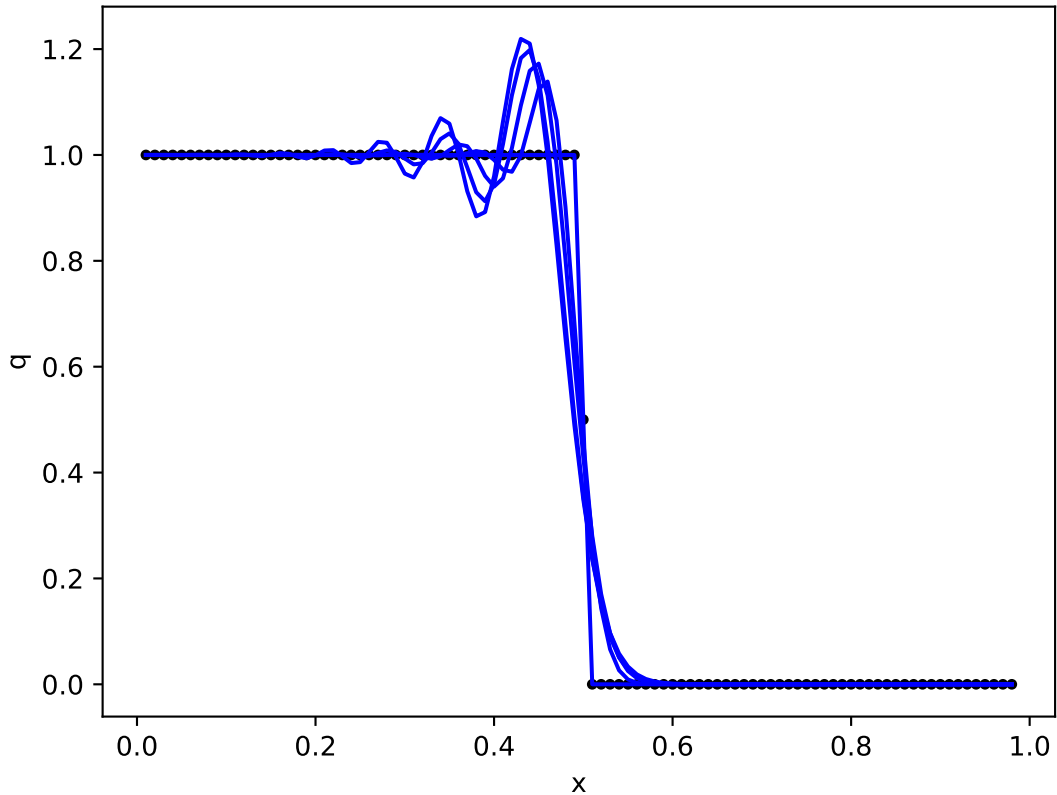
Shock propagation by Lax-Wendroff
