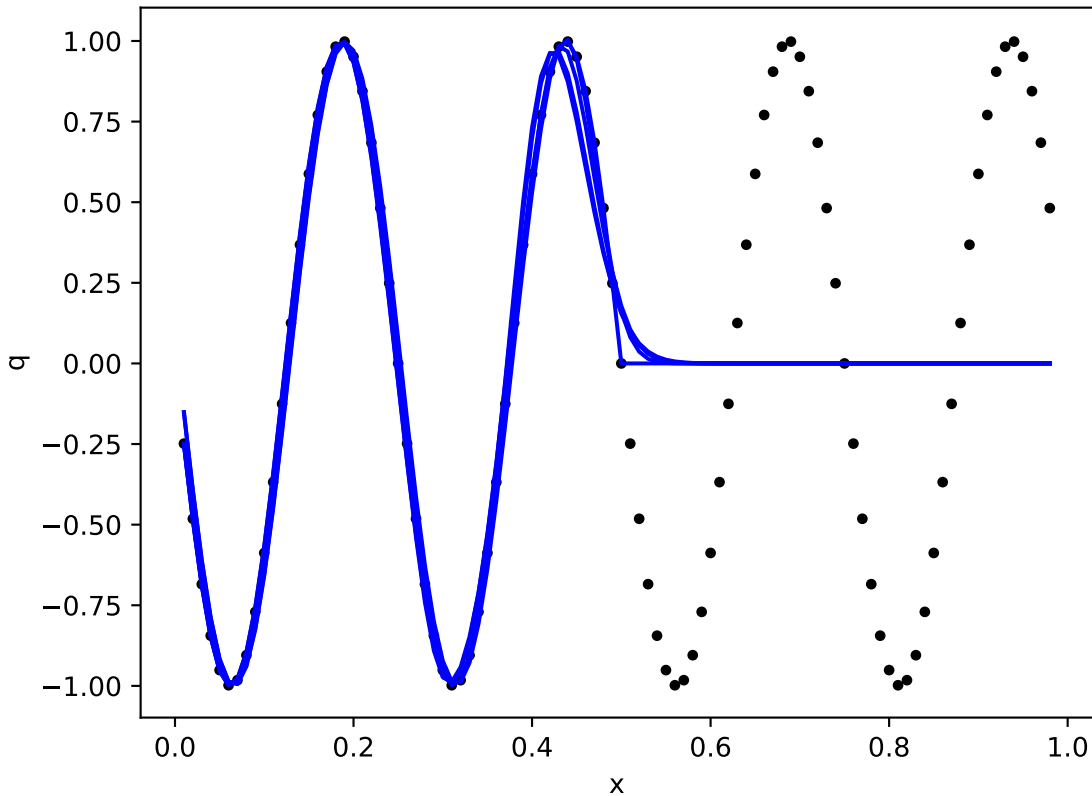
Effect of CFL upon Lax-Wendroff solution of advection equation
