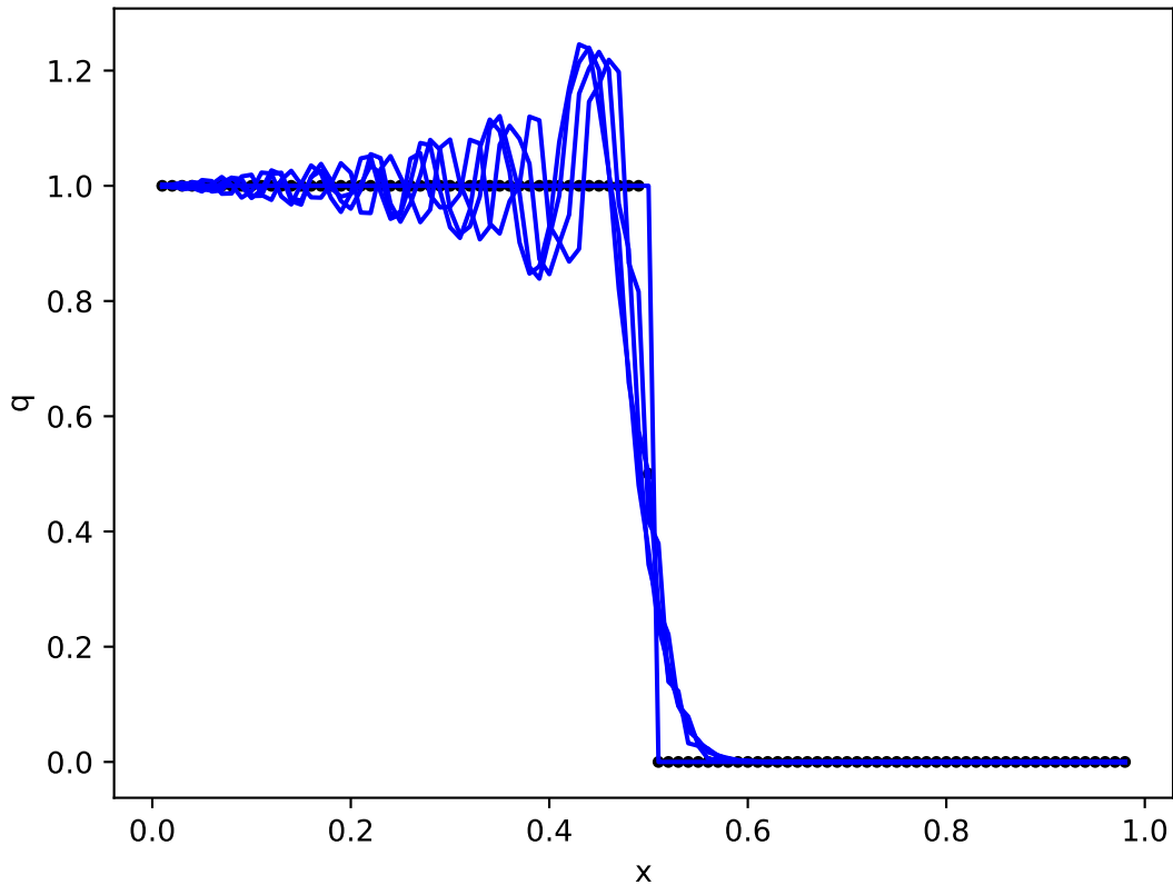
Shock propagation by leap-frog scheme
