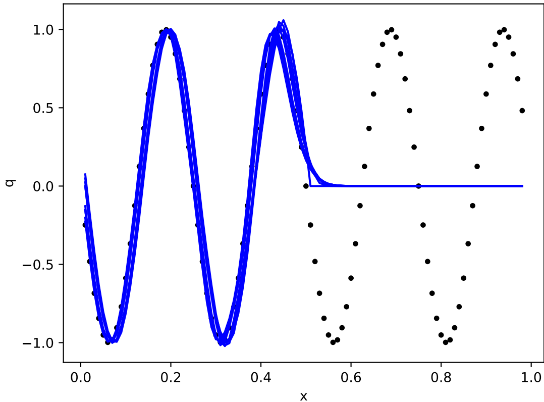
Effect of CFL upon leap-frog solution of advection equation
