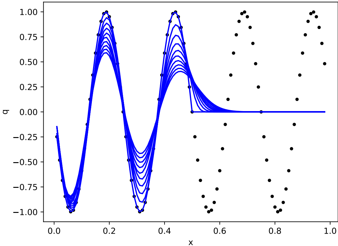
Effect of CFL upon Upwind solution of advection equation
