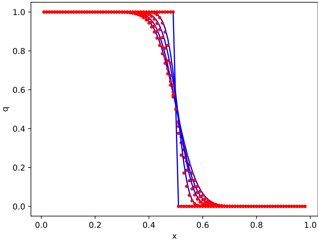
Shock propagation by upwind scheme
